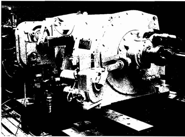
Figure 10. MSVD Multistage Variable Speed Drive, Prototype.
