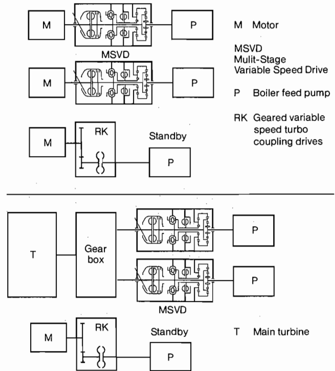
Figure 15. Various Arrangements.
