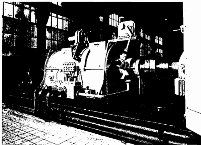
Figure 20. MSVD Compressor Drive, 6800 HP, 3800 RPM.
