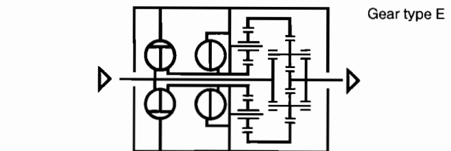
Figure 12. MSVD Design Variants.
