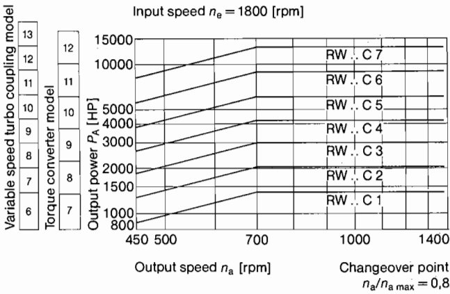
Figure 14. Selection Diagram.
