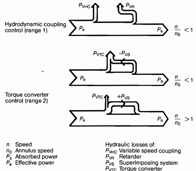
Figure 7. Power Split (Range-Dependent).
