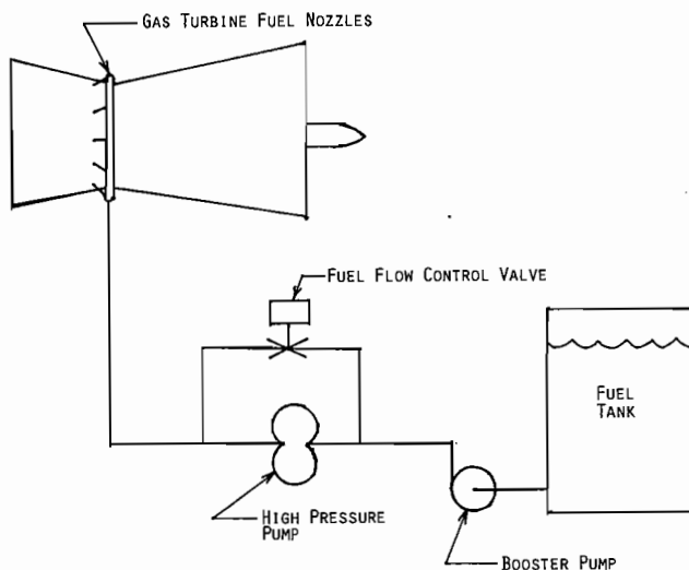
Figure 8. Simplified Gas Turbine Fuel System.
