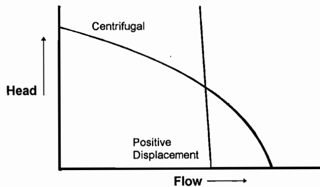
Figure 4. Centrifugal and Positive Displacement Pump Curves.
