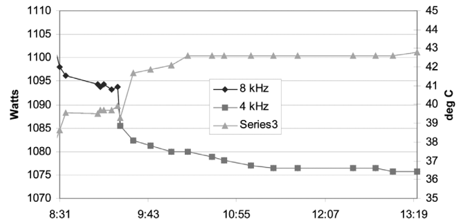
Figure 6. Energy Utilization and Motor Temperature at Several Drive Frequencies.
