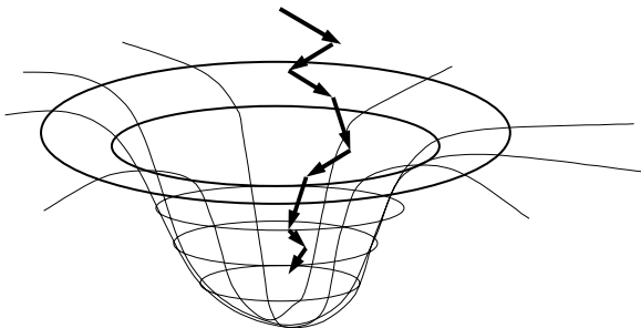
Figure 4. Graphical Representation of Steepest Decent Method.
